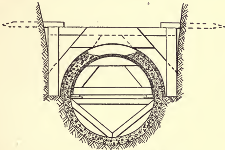
FIG. 26.—FORM FOR CONCRETE ARCH.
